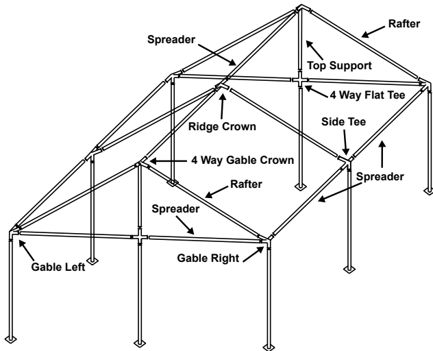
General frame tent construction shown on a 20' x 20'
